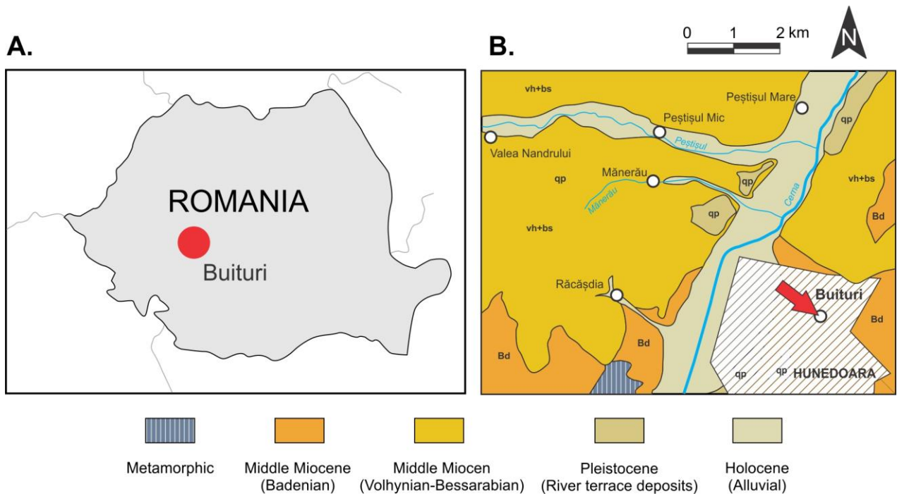
Fig. 1. A. Location of Buituri in Romania; B. Geological map of the Buituri area (after the geological map of the Institute of Geology of Romania 1:50.000, folio Hunedoara, modified and simplified).
